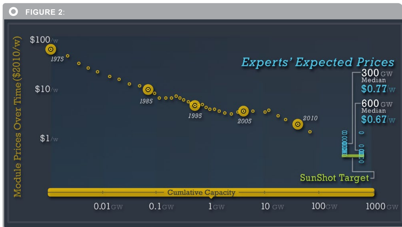
FIGURE 2: Falling prices for solar modules. As the total amount of solar modules produced has increased over the past few decades (from left to right), the price per watt has also fallen. Prices 1975-2009 are from Nemet (2009), and prices for 2010 and 2011 are based on data from Navigant and Bloomberg New Energy Finance. 5 Blue circles indicate the expectations from Near Zero's survey, for solar module prices at 300 GW and 600 GW of total installations (also called cumulative capacity). Also shown for reference in green is the module price target of the Department of Energy's SunShot Program.
